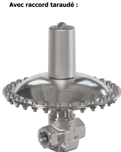
1/2" – 1 1/4"
